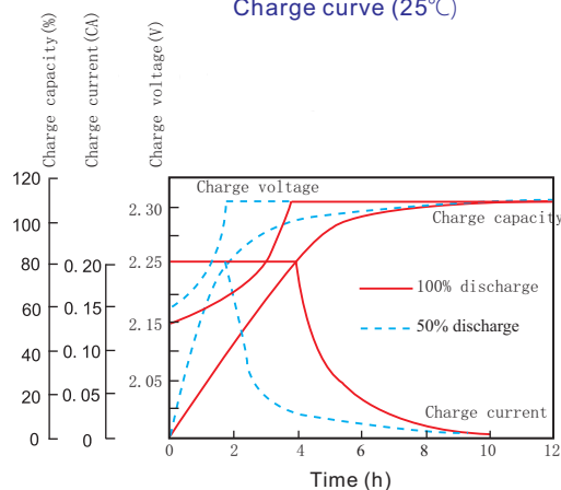
Charge curve (25°C)
