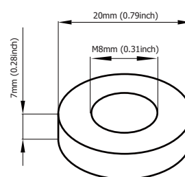
Terminal Dimensions
